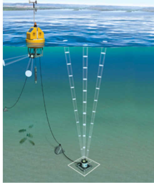
In Sepetiba Bay, HidroMares positioned three bottom-mounted SonTek Argonaut-XR systems in the channel, leading their cables up to surface buoys outfitted with data transmission equipment.
